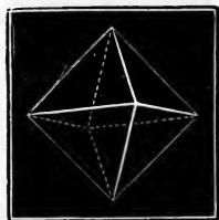
Crystal of Alum.
